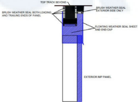
SECTION VIEW TOP WEATHER SEAL
