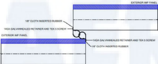
WEATHER SEAL BETWEEN PANELS
