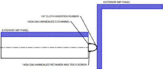
WEATHER SEAL AGAINST ENDWALL
