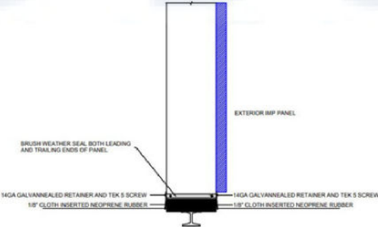
SECTION VIEW BOTTOM WEATHER SEAL
