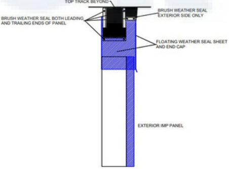
SECTION VIEW TOP WEATHER SEAL
