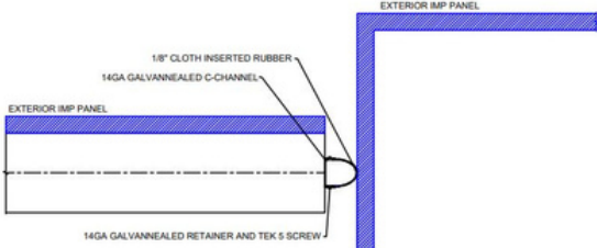
WEATHER SEAL AGAINST ENDWALL
