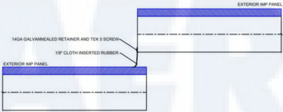
WEATHER SEAL BETWEEN PANELS
